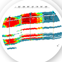
Tracer Modelling
